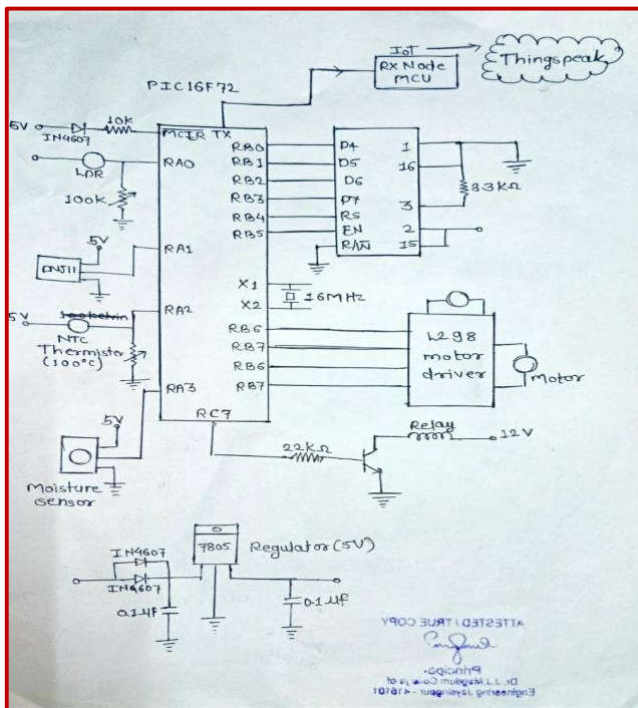
Figure: Block diagram
