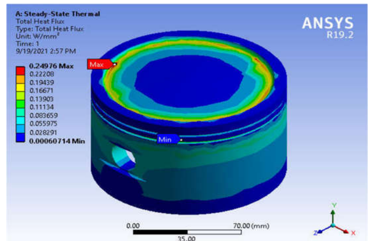
Figure 1.9 – Heat flux distribution of titanium dioxide coated piston.
