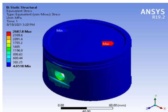
Figure 1.3 thermal stress distributions in piston (Validation)
