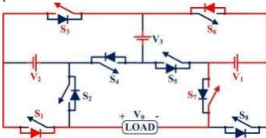
FIGURE 12. Case-7 for the 15MLI.
