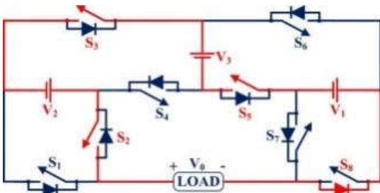
FIGURE 15. Case-10 for the 15MLI.
