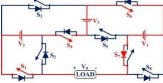
FIGURE 19. Case-14 for the 15MLI.
