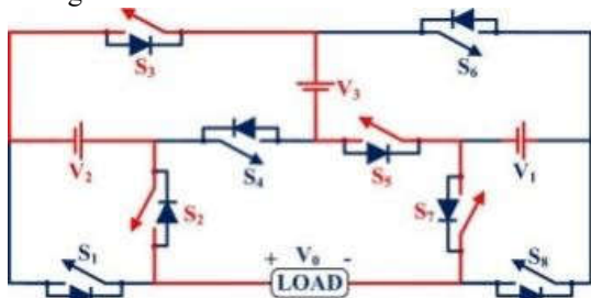
FIGURE 6. Case-1 for the 15MLI
