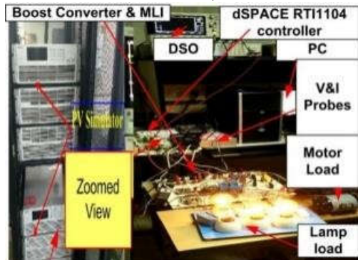
FIGURE 26. Prototype model of 15MLI.
