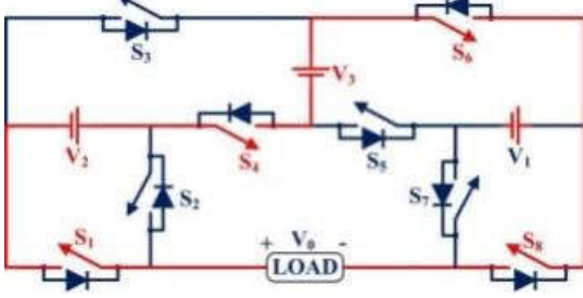
FIGURE 20. Case-15 for the 15MLI.
