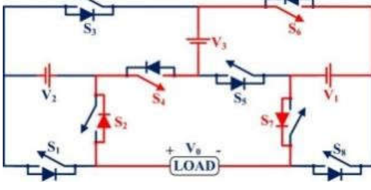
FIGURE 17. Case-12 for the 15MLI.
