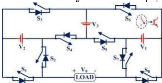
FIGURE 5. Proposed topology of 15 levels.
