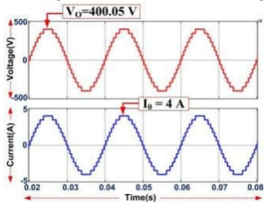
FIGURE 23: The 15MLI's two-cycle output waveform.
