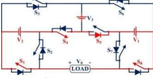
FIGURE 16. Case-11 for the 15MLI.
