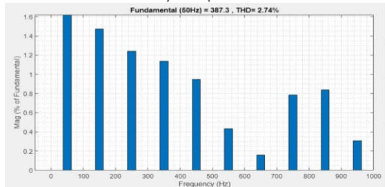
FIGURE 24. The 15MLI THD simulation.
