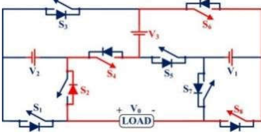
FIGURE 18. Case-13 for the 15MLI.
