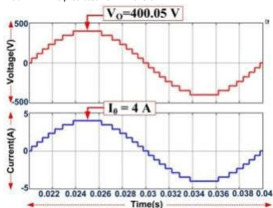
FIGURE 22. The 15MLI's single-cycle output waveform.
