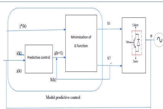
Fig.3 Schematic representation of Model predictive control
