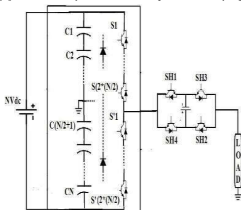
Fig1. Diode Clamped Multilevel Inverter DC-MLI
