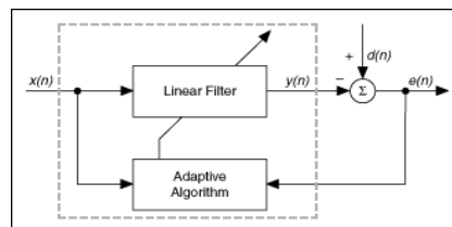
Fig 4: Structure of Adaptive filter
