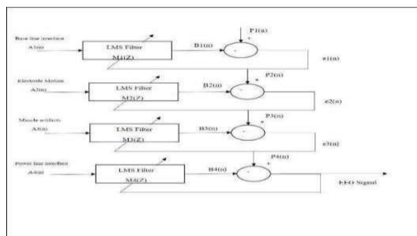
Fig 5: Block Diagram
