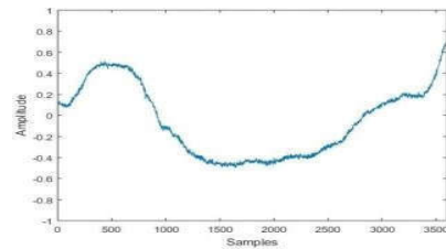
Fig 6.5 Baseline Artifacts
