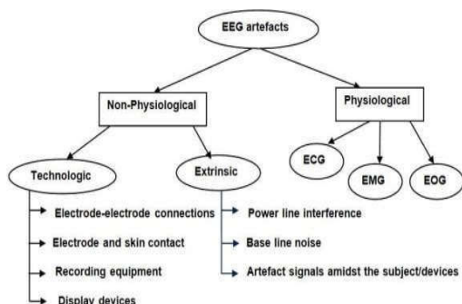
Fig 2: EEG Artifacts
