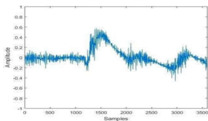
Fig 6.18: Muscle motion Artifacts
