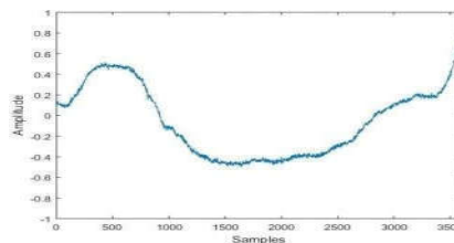
Fig 6.16 Baseline Artifacts
