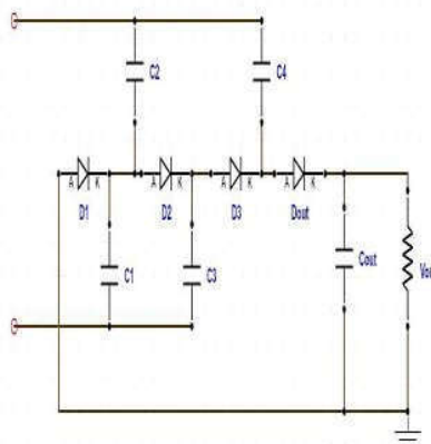
Figure 3.1. Modified Dickson Charge Pump
