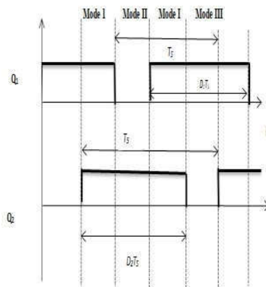
Figure 4.4 Switching signals for the switches Q1 & Q2 of modified Dickson charge converter
