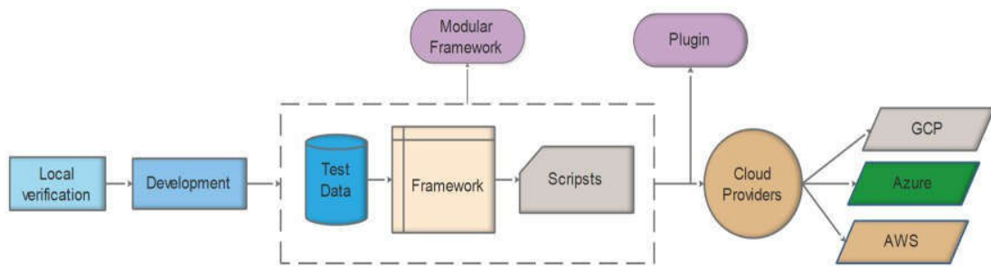
Figure5: proposed Framework of Continuous Testing Modular Framework
