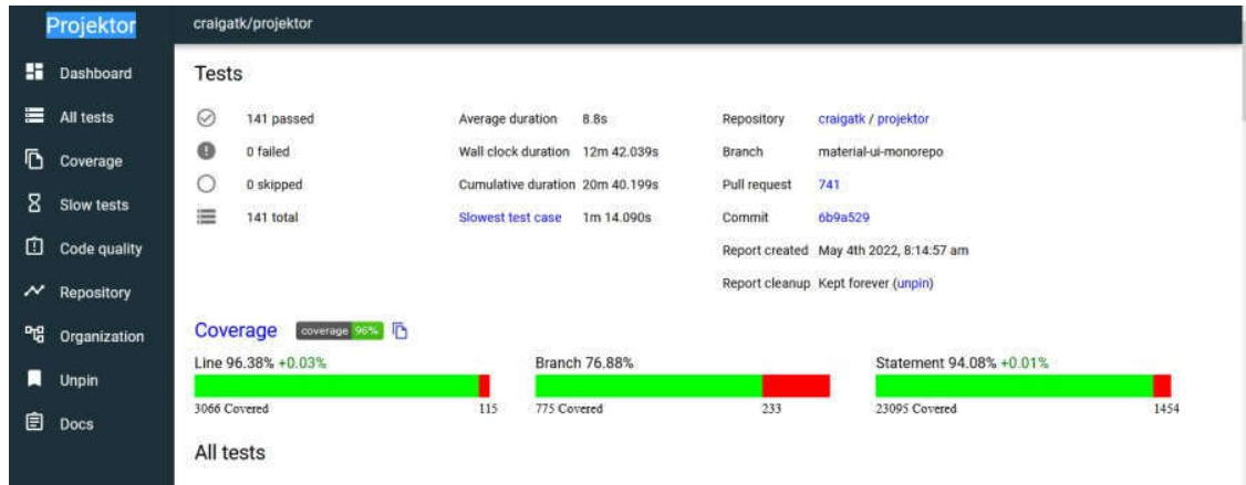
Diagram: projektor Coverage Report
