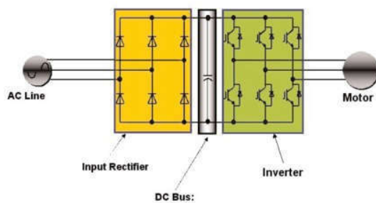
Fig. 3.2. VFD basics: Existing technology
