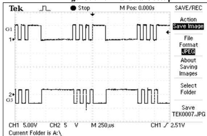
Figure 10: Gating pulse of switch S1 and S3.
