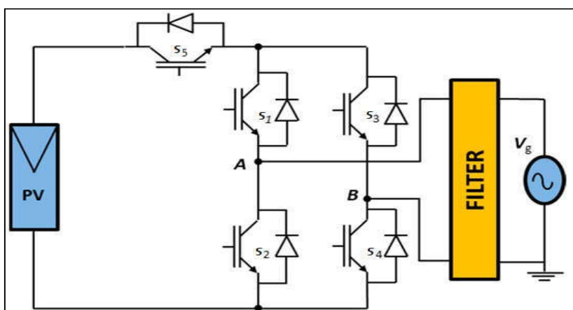
Figure 3: H5 SST inverter topology
