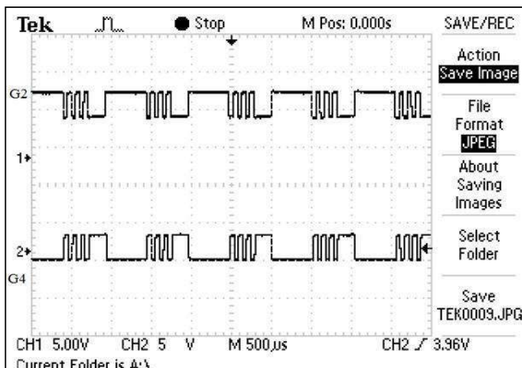
Figure 11: Gating pulse of switch S2 and S4.
